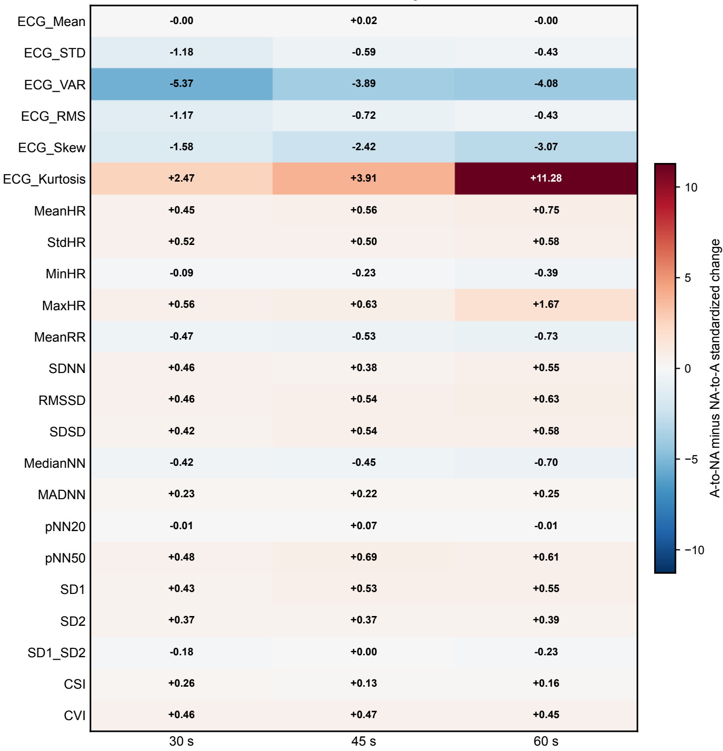
Feature-level direction effects after global FDR control
